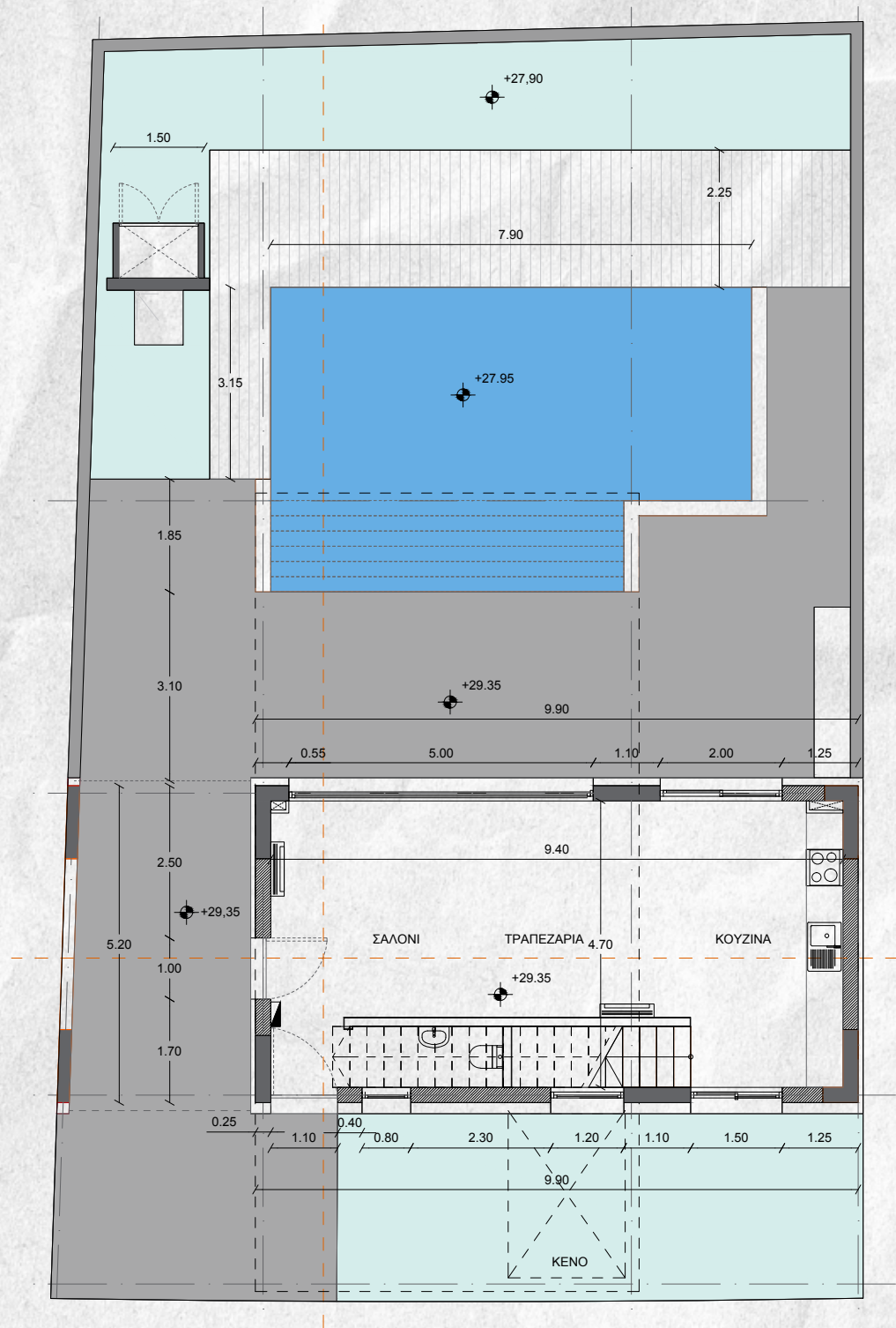
GROUND FLOOR
