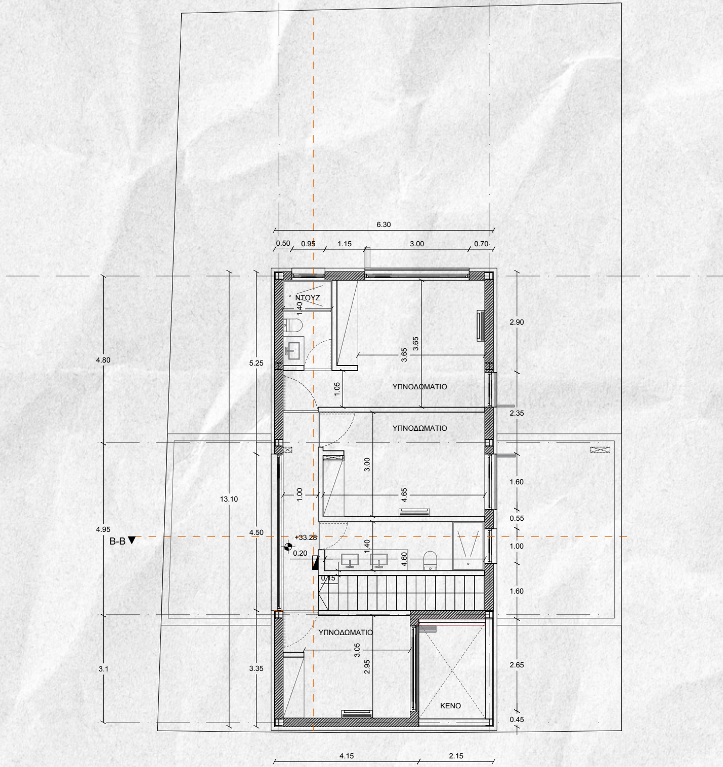
FIRST FLOOR
